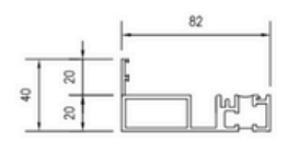
Low Threshold with Rebate - No Cill
